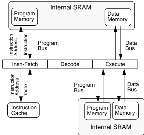
Figure 1: SHARC pipeline
