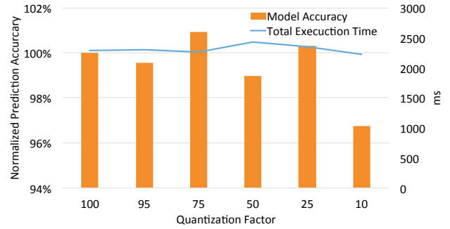
Fig. 8: Effects of JPEG compression on prediction accuracy. Runtime values based on the Caltech dataset images.
