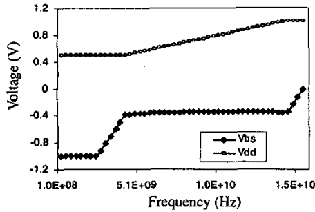
Fig. 5. Plot of the V_{dd} and V_{bs} values for optimal energy reduction in a 50\mu s duration low-power state.
