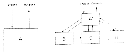
Figure 4. Interface Task
