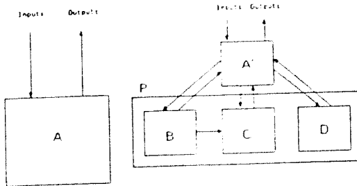
Figure 5 Task Partitioning
