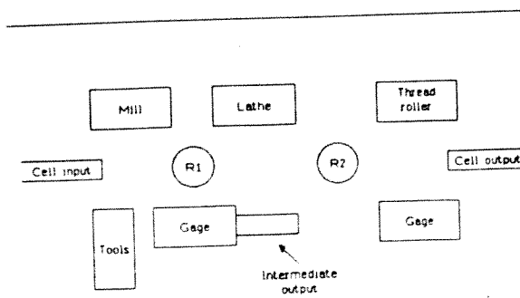
Figure 11: Machining Cell
