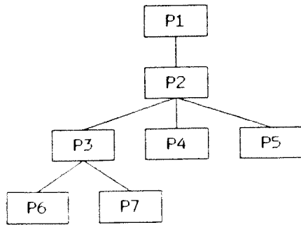
Figure 6 Package Tree
