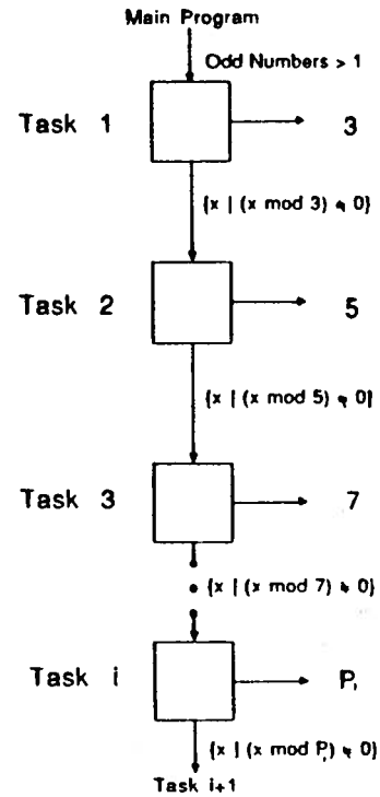
Figure 1: Task pipeline.
